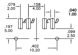
PCB MOUNTING
