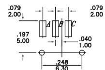
PCB MOUNTING
