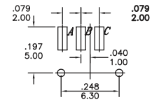
PCB MOUNTING
