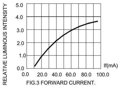
FIG.3 FORWARD CURRENT.
